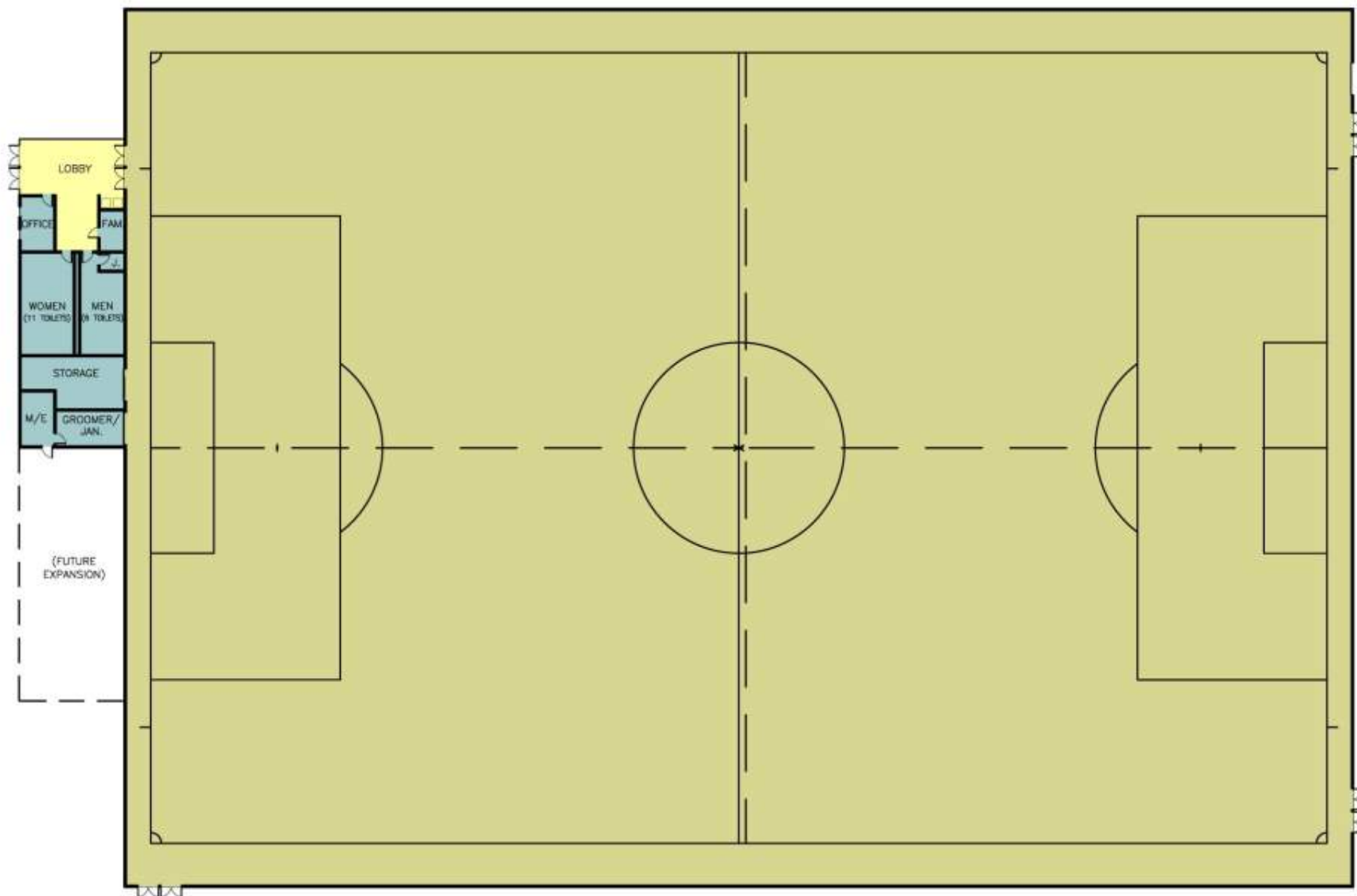
Overall Floor Plan 1/32" = 1'-0"
